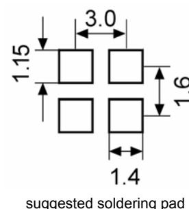
suggested soldering pad
